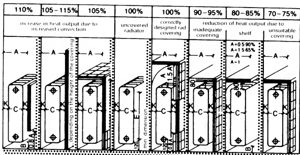
1 Variation of heat output for various heater/covering combinations
